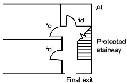
Diagram 2 Alternative arrangements for final exits
