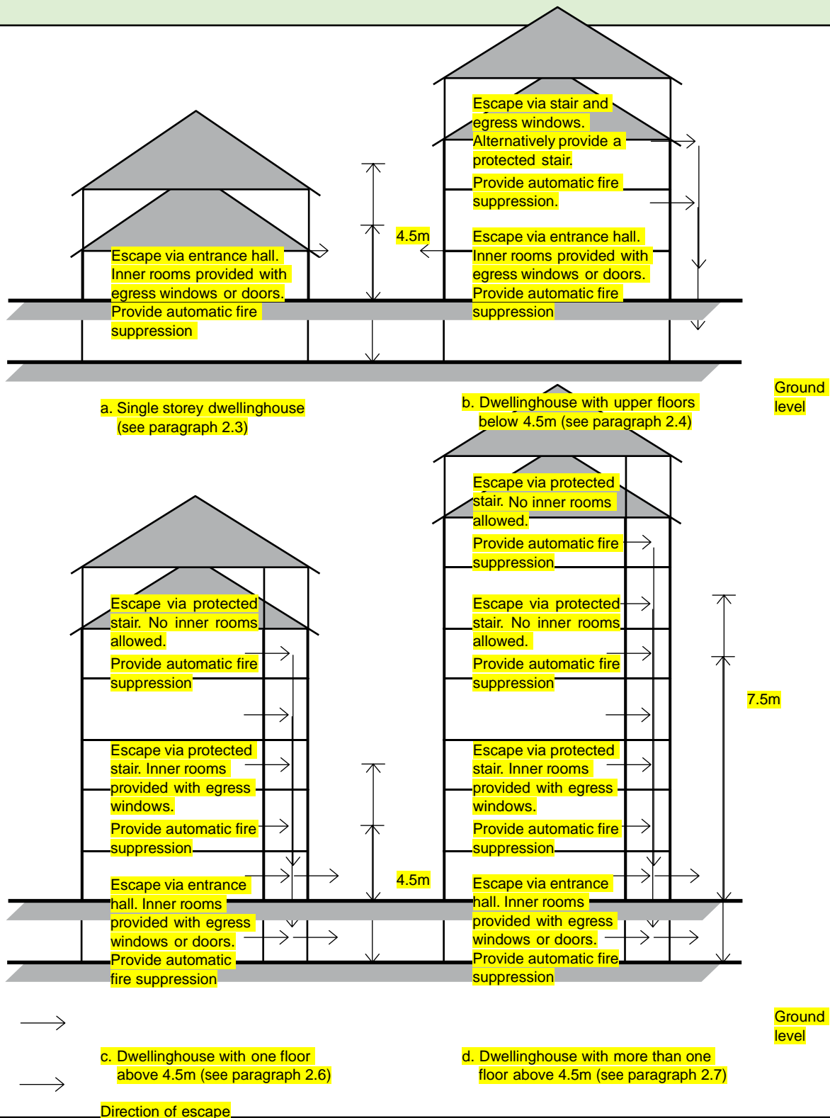
Diagram 1 Means of escape from dwellinghouses
