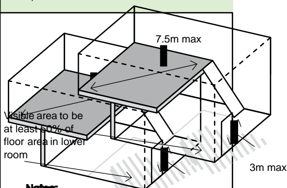
Diagram 5 Gallery floors with no alternative exit
