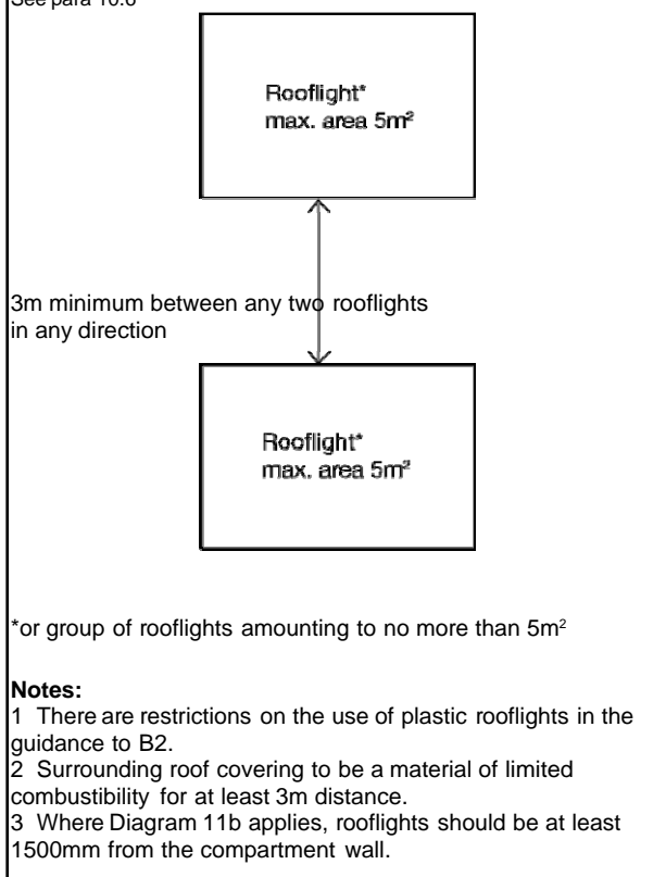
Diagram 23 Limitations on spacing and size of plastic rooflights having a Class 3 (National class) or Class D-s3, d2 (European class) or TP(b) lower surface
