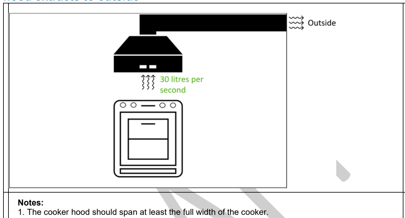
Diagram 1.2 – Minimum ventilation rate for kitchen extract where cooker hood does not extract to outside 1
