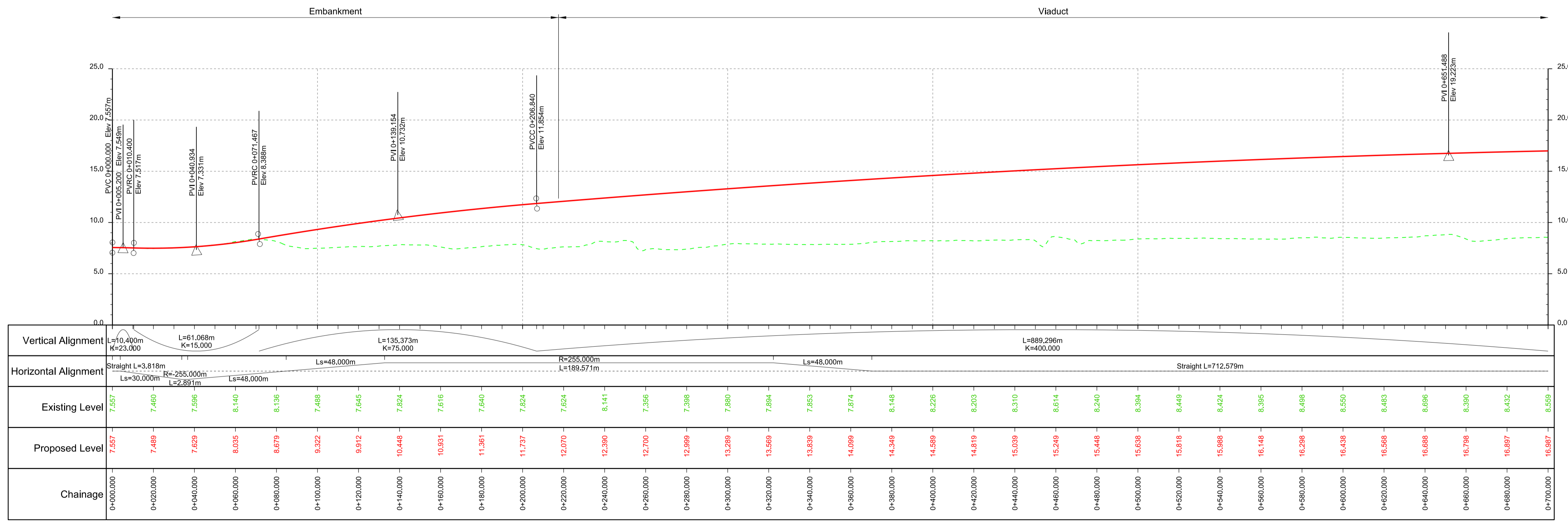
Mainline A487 Profile
