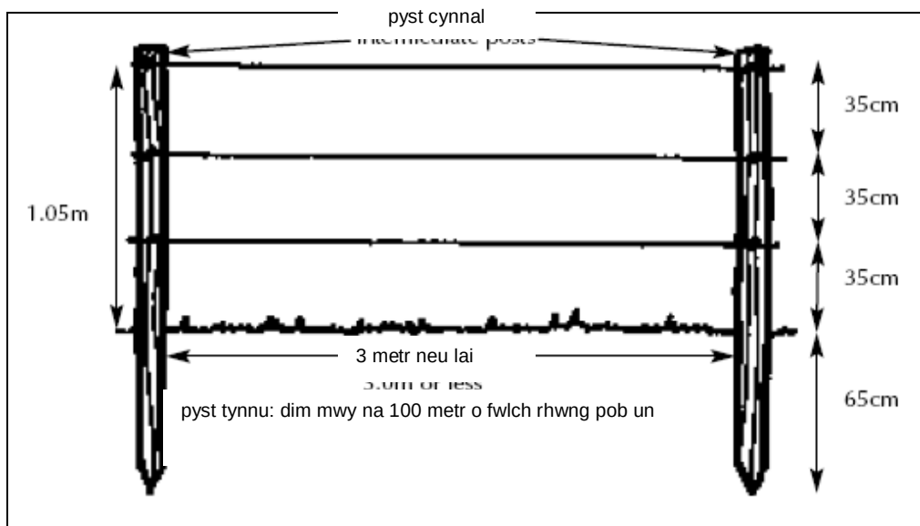
Diagram o ffens tair gwifren
