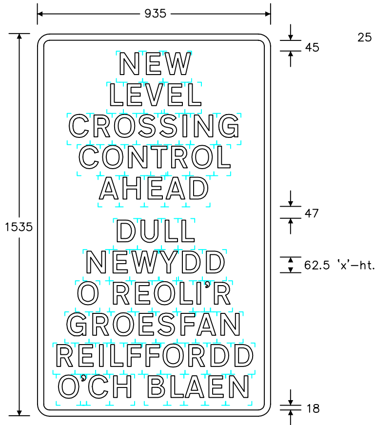
Sign for railway level crossing
