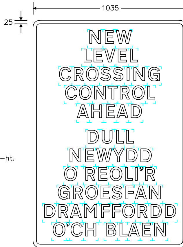
Sign for tramway level crossing
