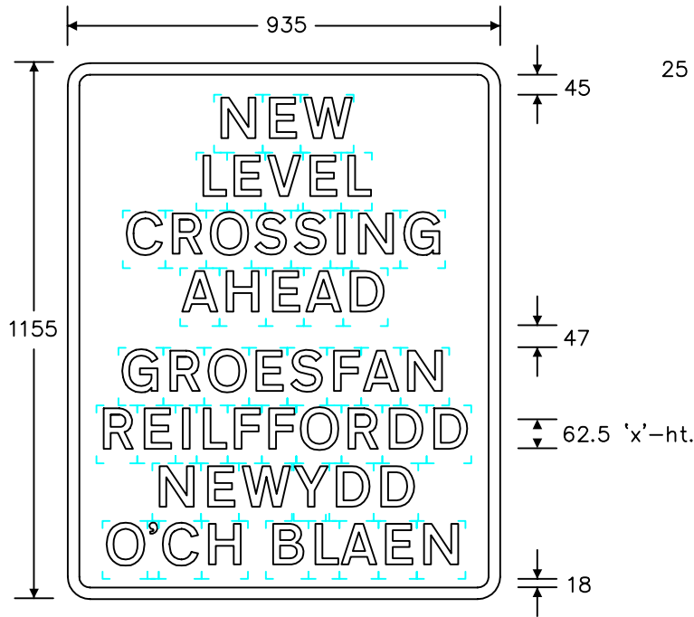
Sign for railway level crossing
