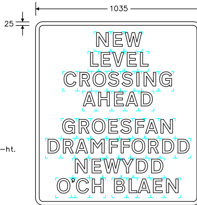
Sign for tramway level crossing
