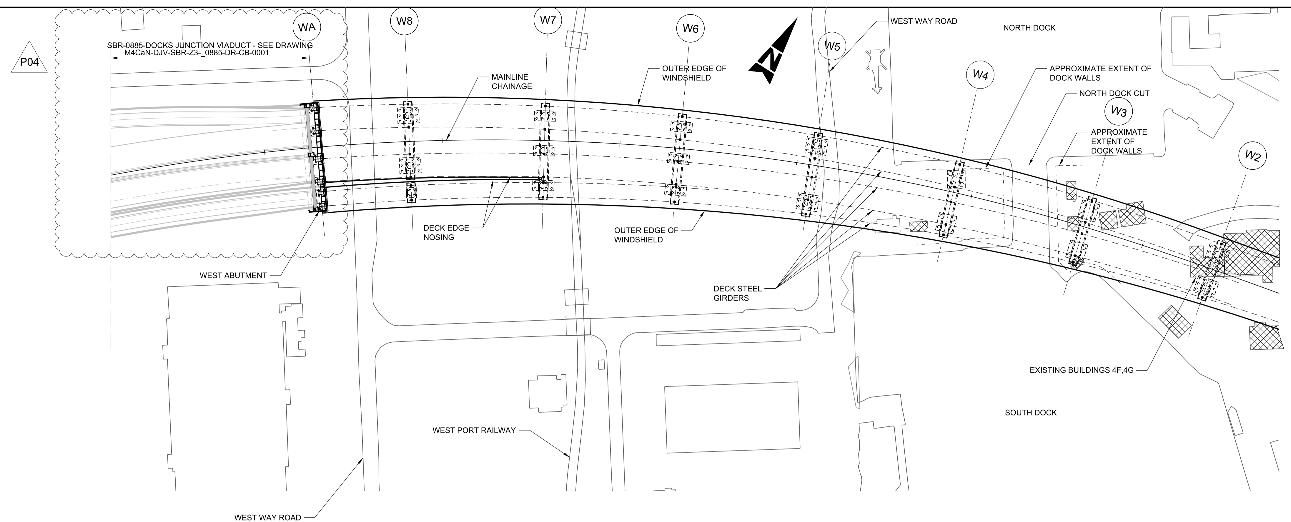
PLAN Scale 1:250
