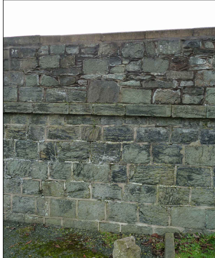
CAR PARK RETAINING WALL: DRESSED MASONRY BLOCKS, COURSED AND UNCOURSED
