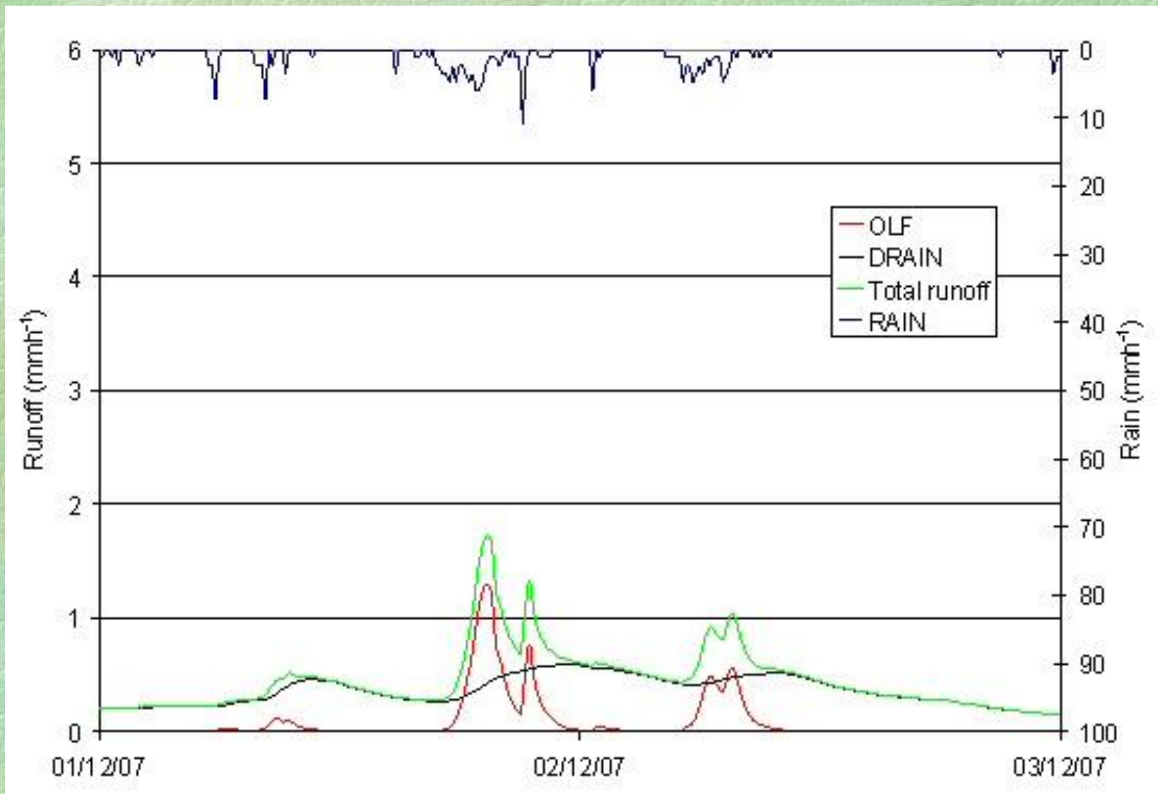
Runoff response from the bowl study site for the period 01/12/07 – 03/12/07.
