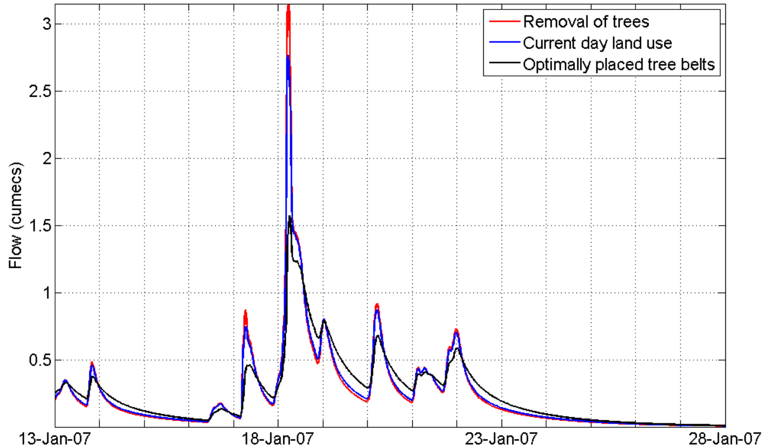
Flow at Pontbren Stream gauge 7
