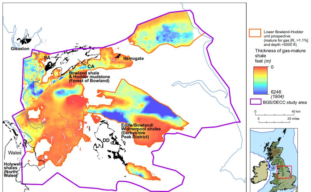
Figure 6 Thickness and distribution of lower Bowland-Hodder unit which are within the gas window and at greater than 1524m (5000ft) (Andrews, 2013a)
