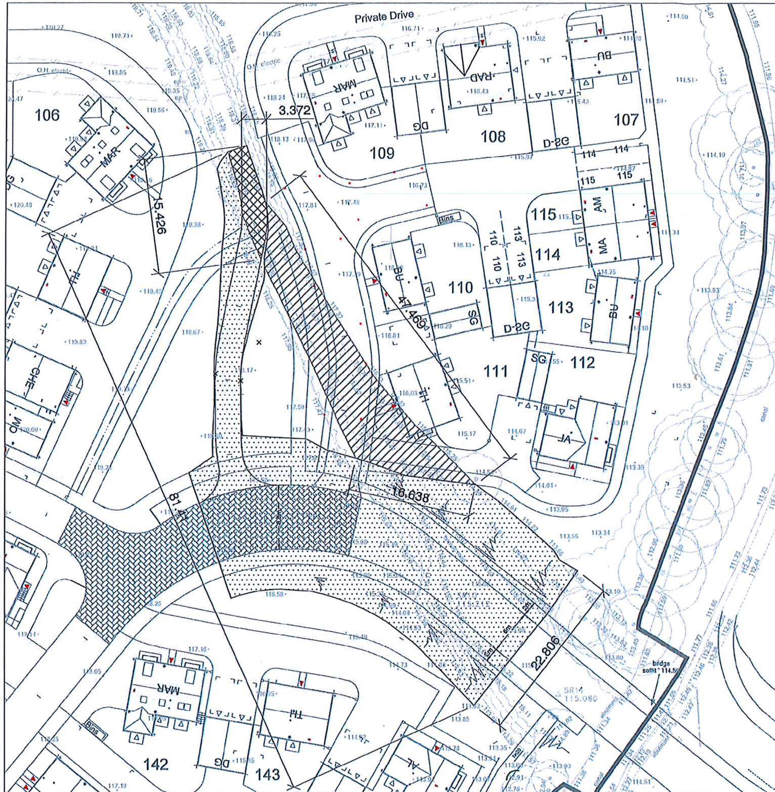
General Arrangement - Stopping Up Order - Bevans Lane (Graddfa / Scale - 1:500)
