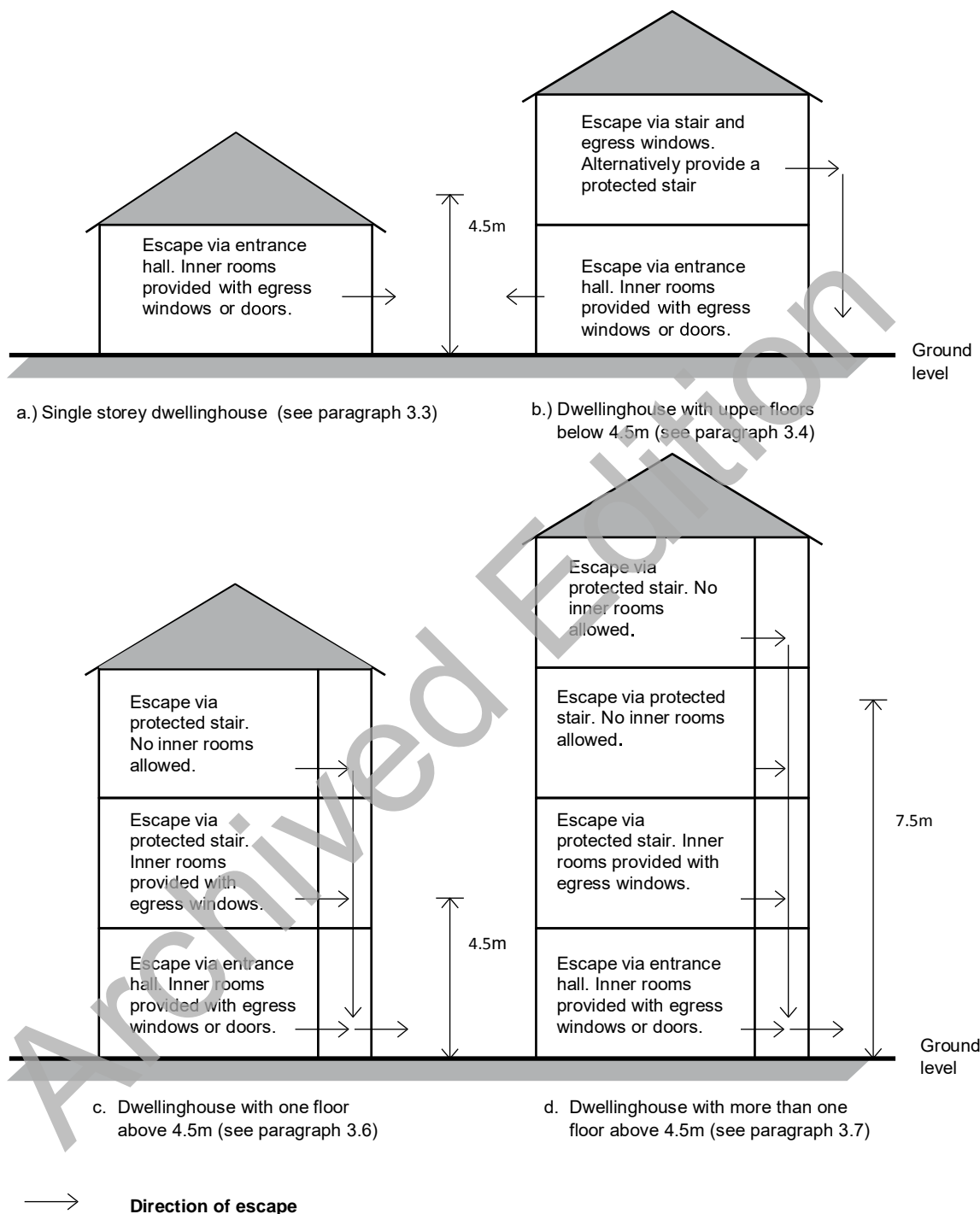
Diagram 1 Means of escape from dwellinghouses
