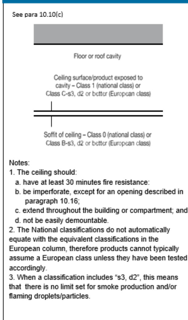
Diagram 35 Fire-resisting ceiling below concealed space
