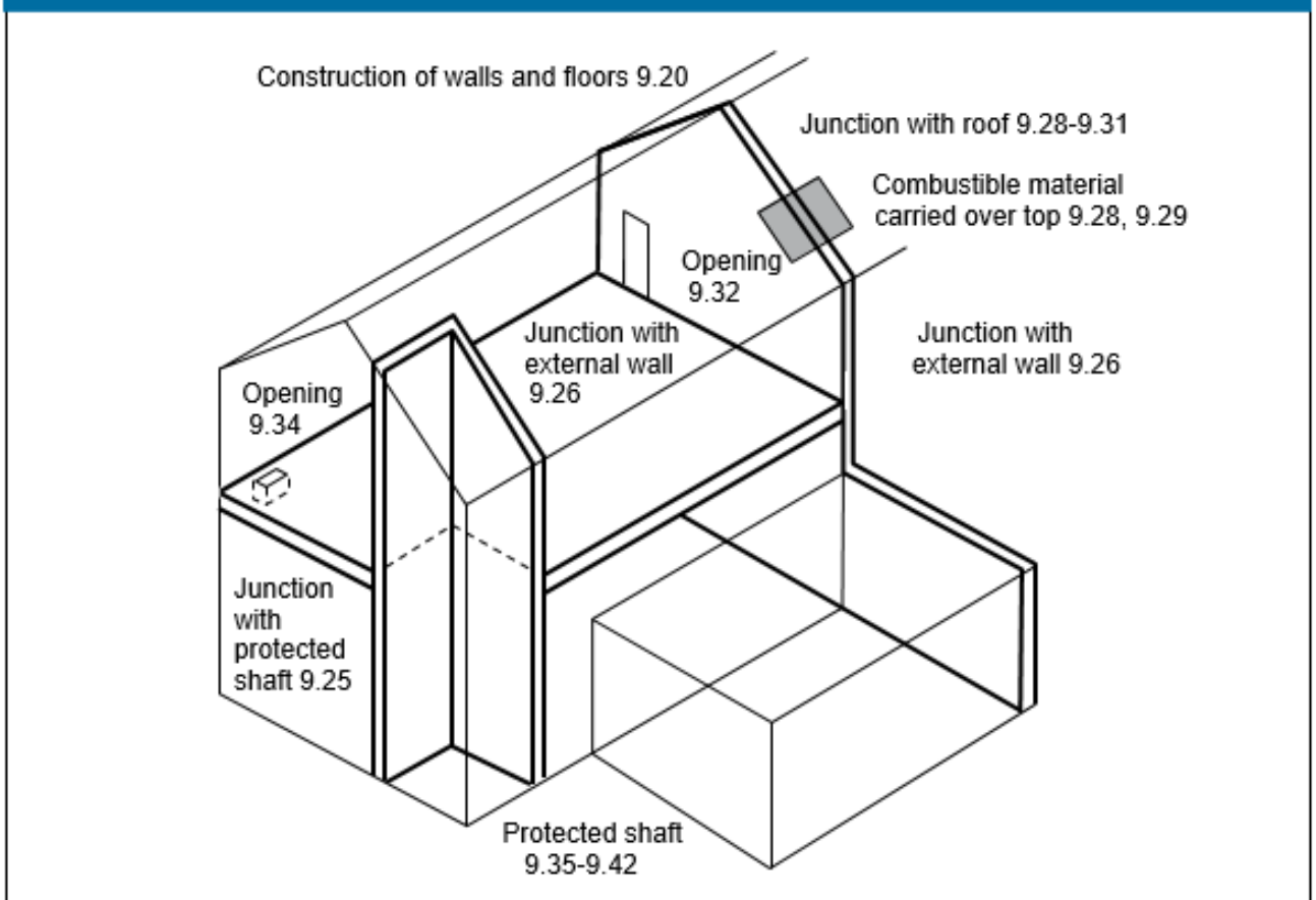
Diagram 29 Compartment walls and compartment floors with reference to relevant paragraphs in Section 9
