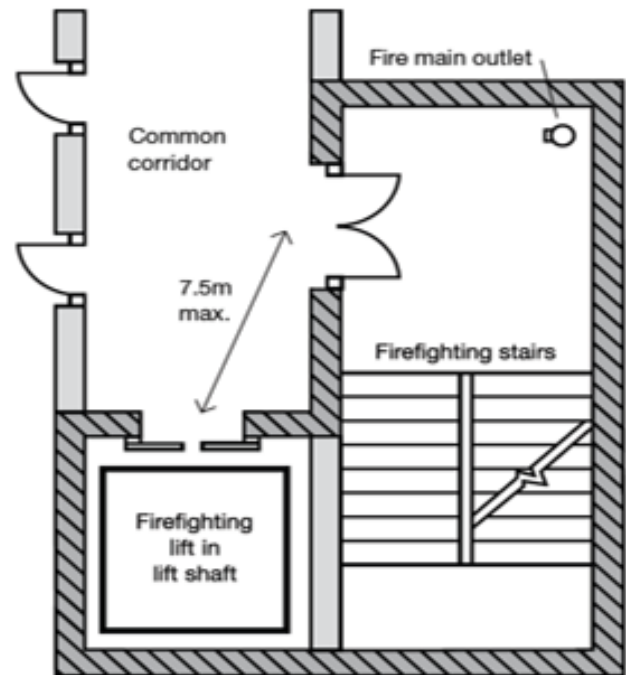
b. Shafts serving flats
