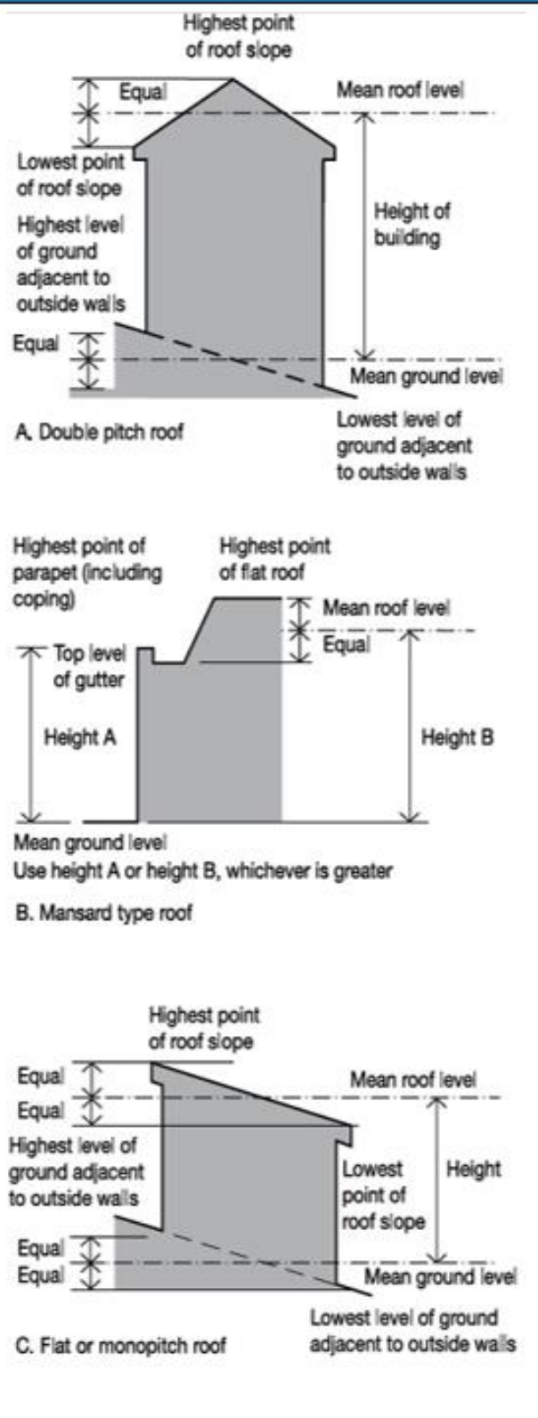
Diagram C4 Height of building
