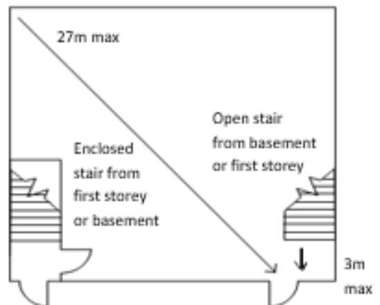
c. BASEMENT
