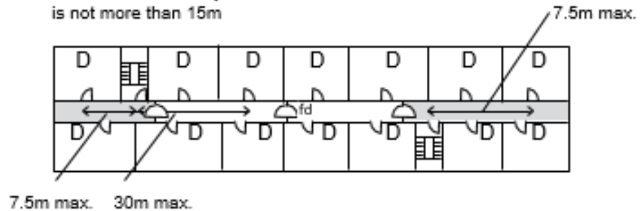
b. CORRIDOR ACCESS WITH DEAD ENDS
