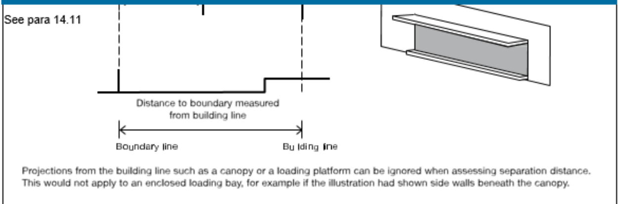
Diagram 45 The effect of a canopy on separation distance
