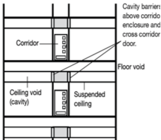
a. SECTION TO SHOW USE OF CAVITY BARRIERS ABOVE THE CORRIDOR ENCLOSURE see paragraph 4.26 a.
