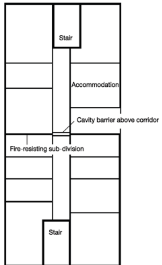
b. PLAN SHOWING SUB-DIVISION OF THE STOREY BY FIRE-RESISTING CONSTRUCTION See paragraph 4.26 b
