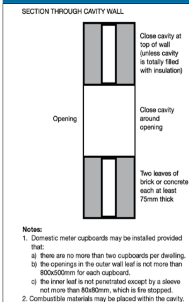
Diagram 34 Cavity wall excluded from provisions for cavity barriers
