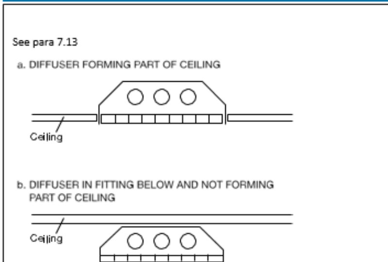
Diagram 26 Lighting diffuser in relation to ceiling
