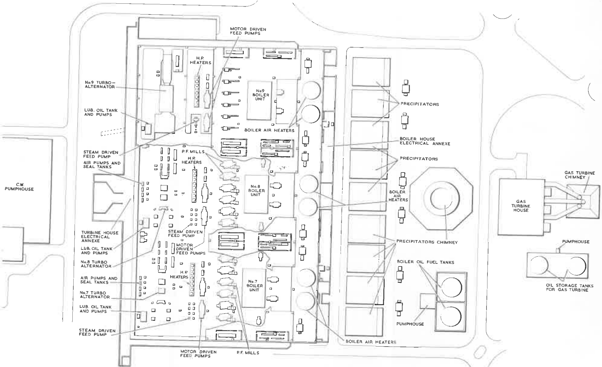
MAIN PLANT LAYOUT - PLAN
