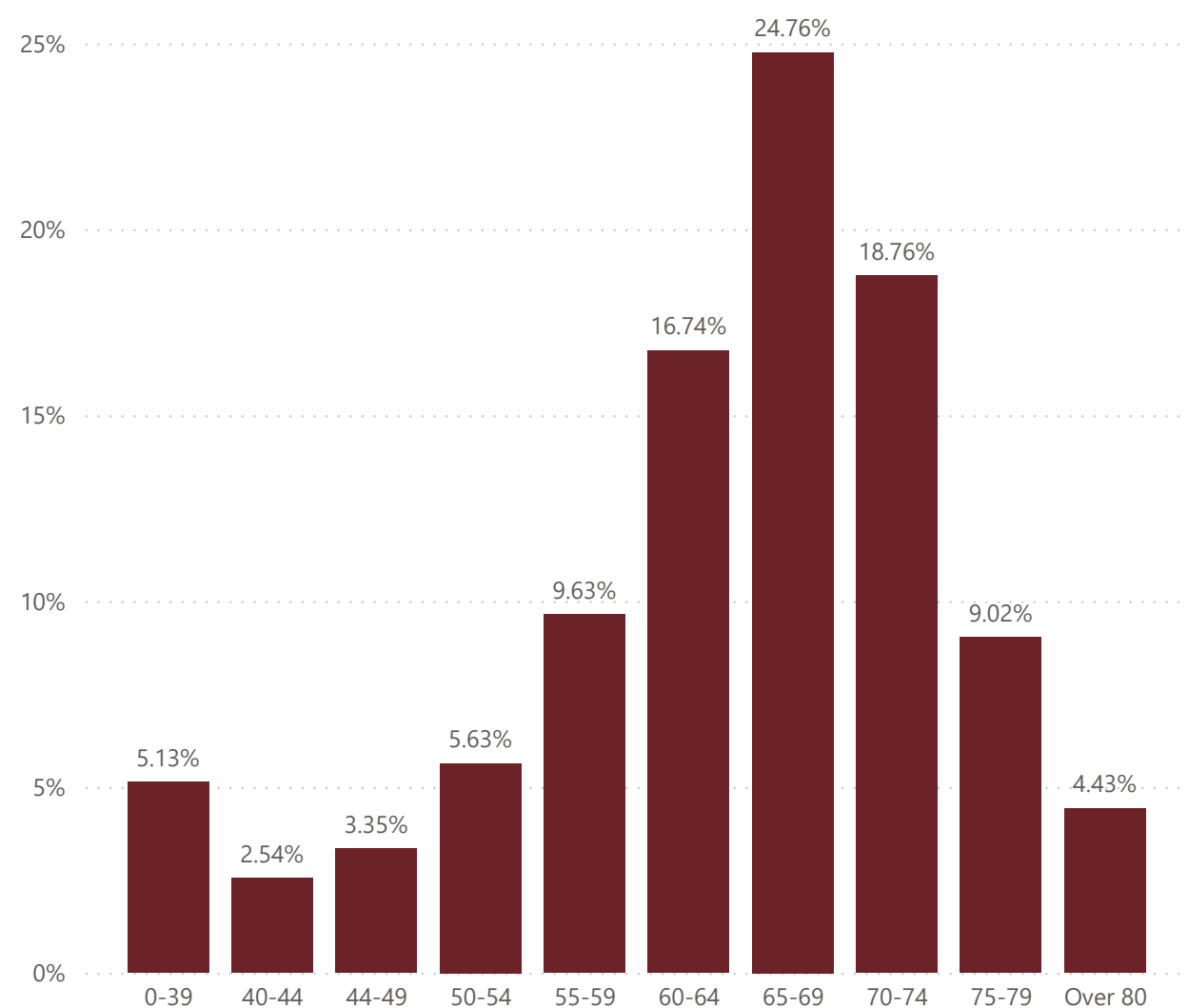
Southbound Traffic Speed Profile (partial years data)
