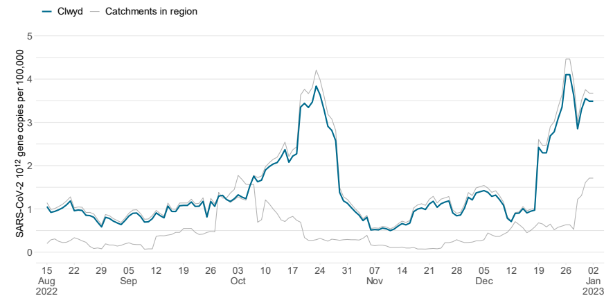
Figure 12 - Regional mean (blue lines) Site mean (grey lines) SARS-CoV-2 gc/day per 100k
