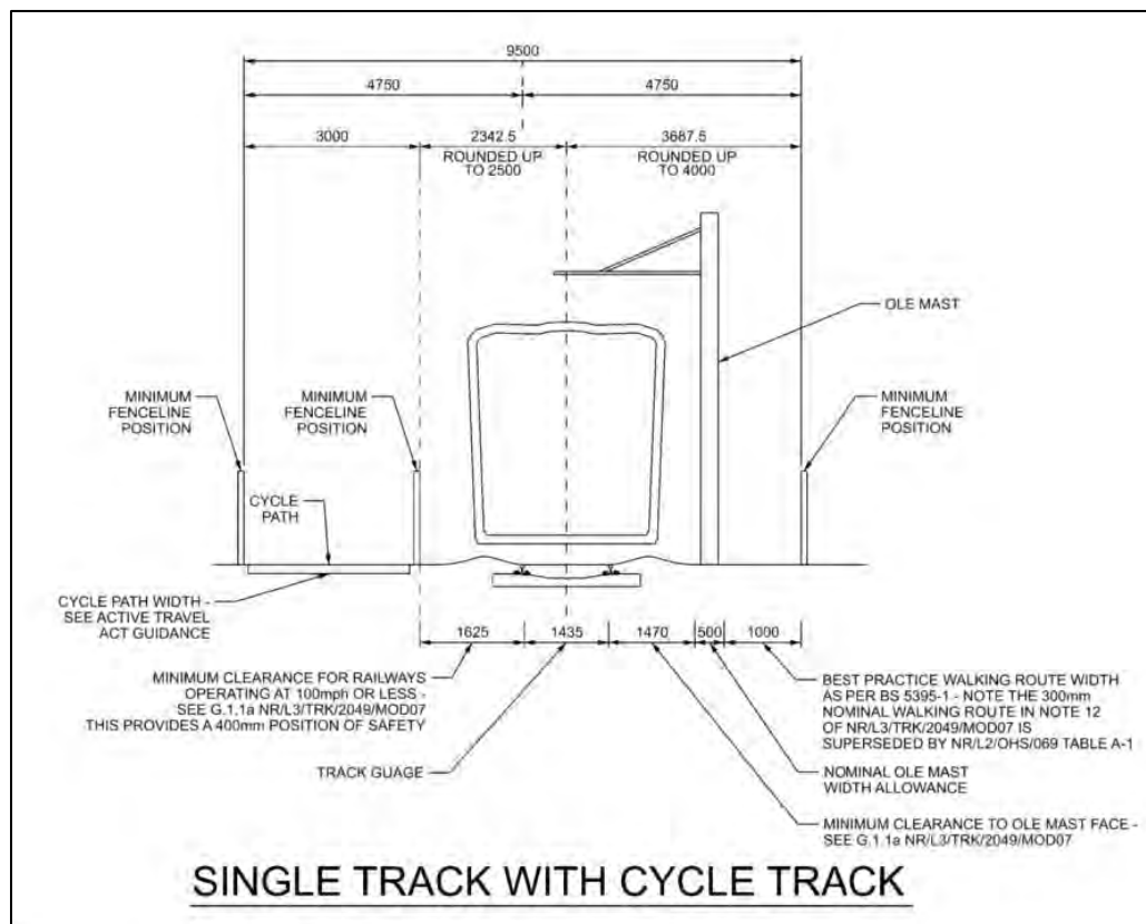
Figure 4-4 – Proposed Safeguarded corridor cross section - single track with adjacent cycle track
