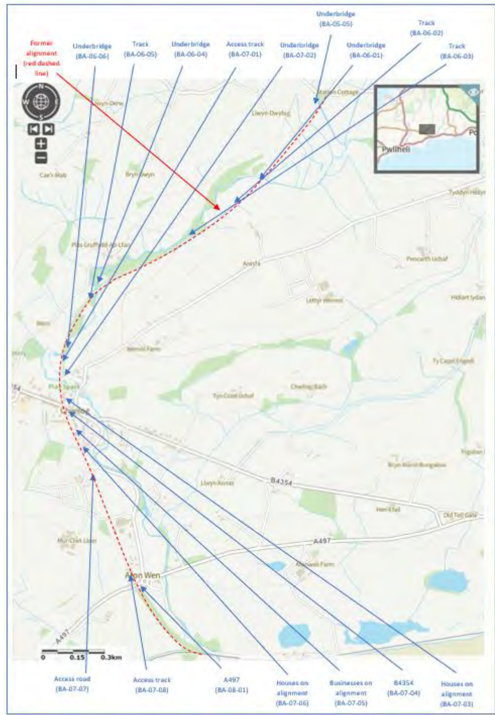
Figure 11-25 – Overview of Former Llangybi Station to Afon Wen showing obstructions along the route
