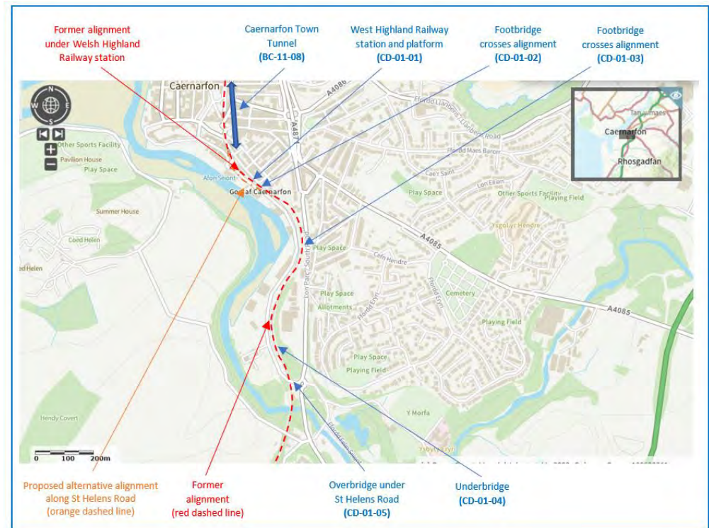
Figure 8-1 – Overview of Caernarfon Tunnel to Pont Seiont Roundabout showing the obstructions along the route
