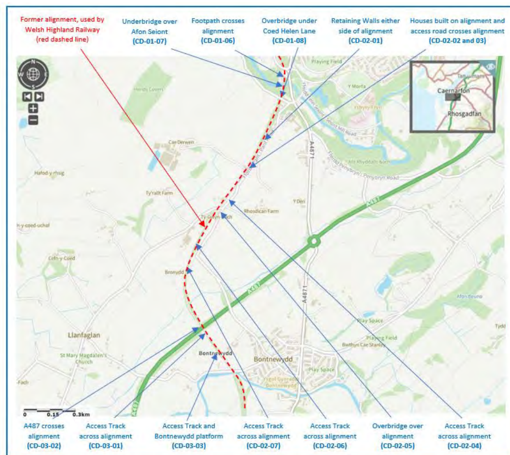
Figure 8-13 – Pont Seiont Roundabout to Bontnewydd Halt showing the obstructions along the route
