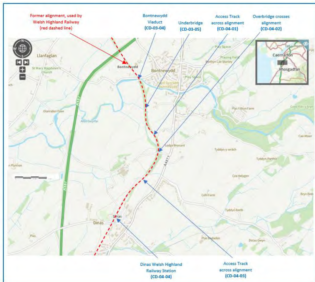
Figure 8-25 –Bontnewydd Halt to Dinas Station showing the obstructions along the route
