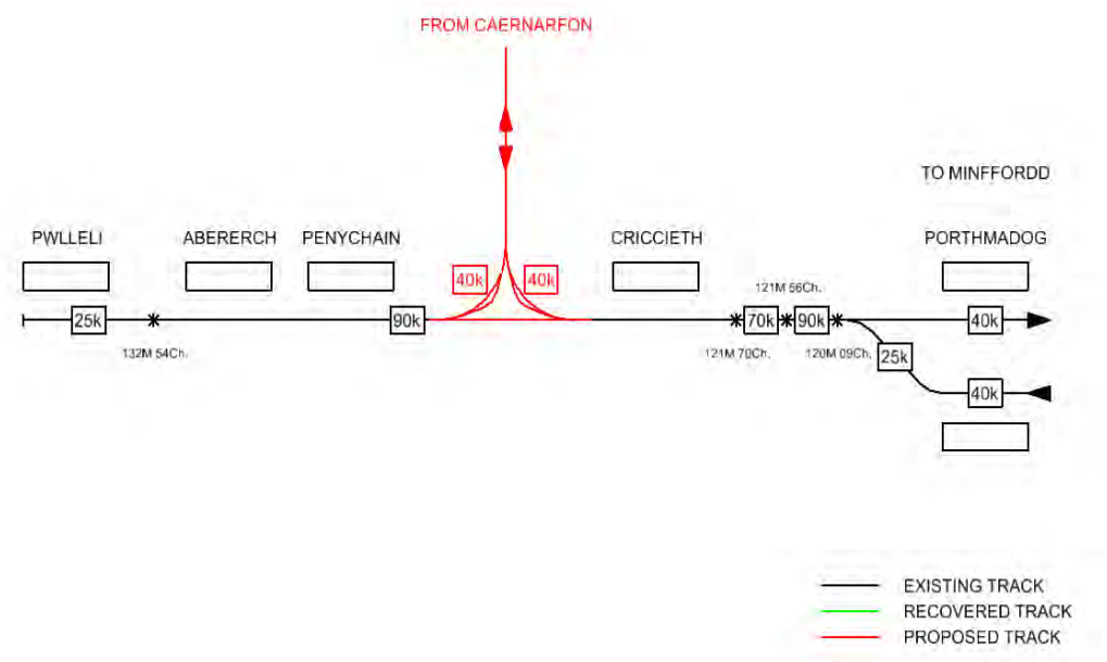
Figure 6-10 - Proposed Line Diagram
