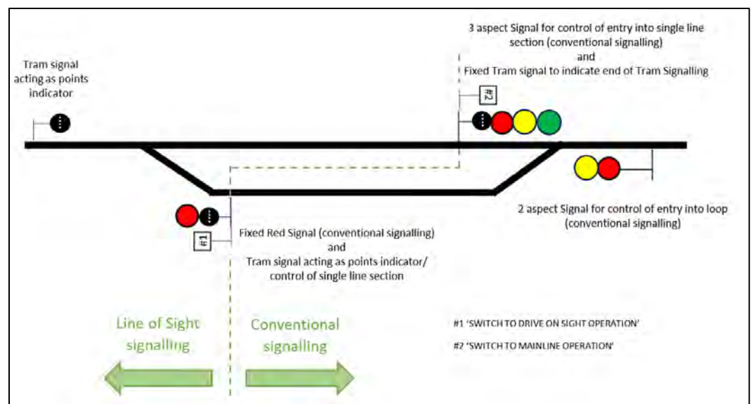
Figure 4-2 – Transition between tram and train mode
