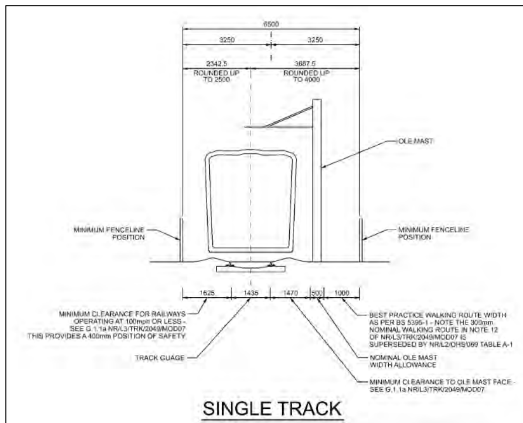
Figure 4-3 - Proposed Safeguarded corridor cross section - single track
