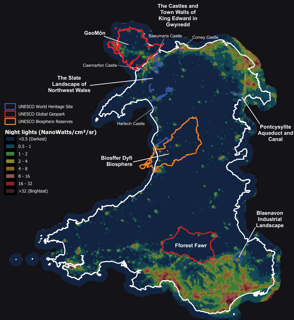
NRW Dark skies satellite data with all UNESCO World Heritage Sites, Biosphere and Global Geoparks
