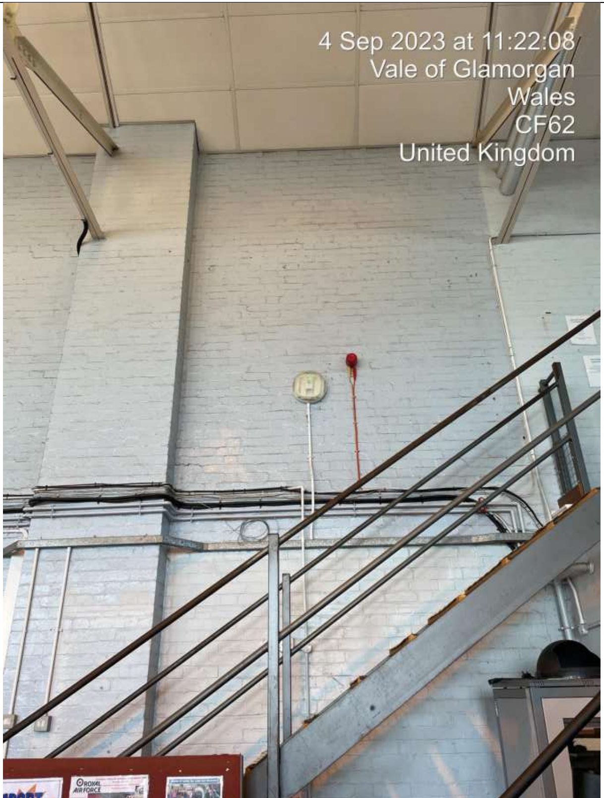
Penetrating Damp & Unprotected Cable Installations.
