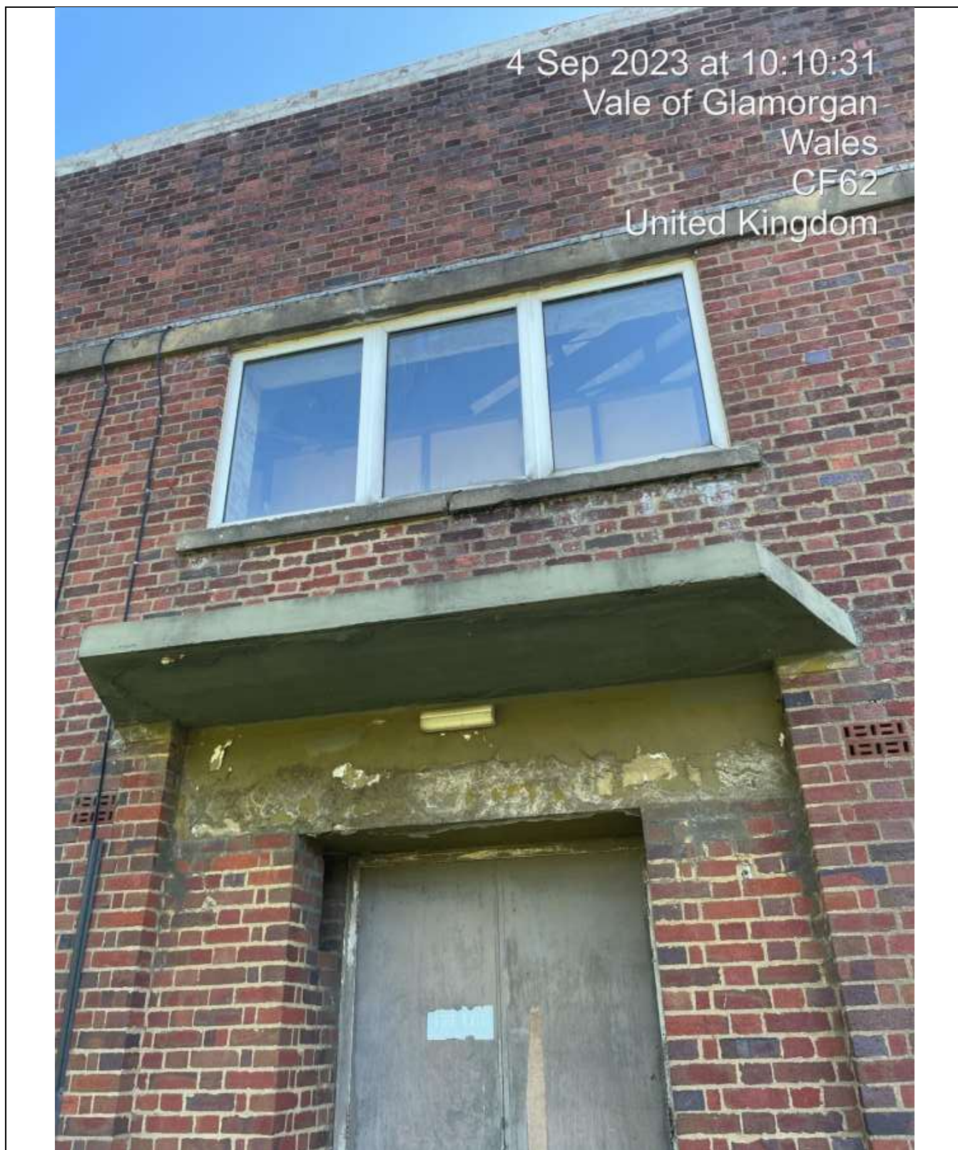
Western Elevation. Deterioration to Doors. Poor Patching Repair to Concrete Lintel Over.
