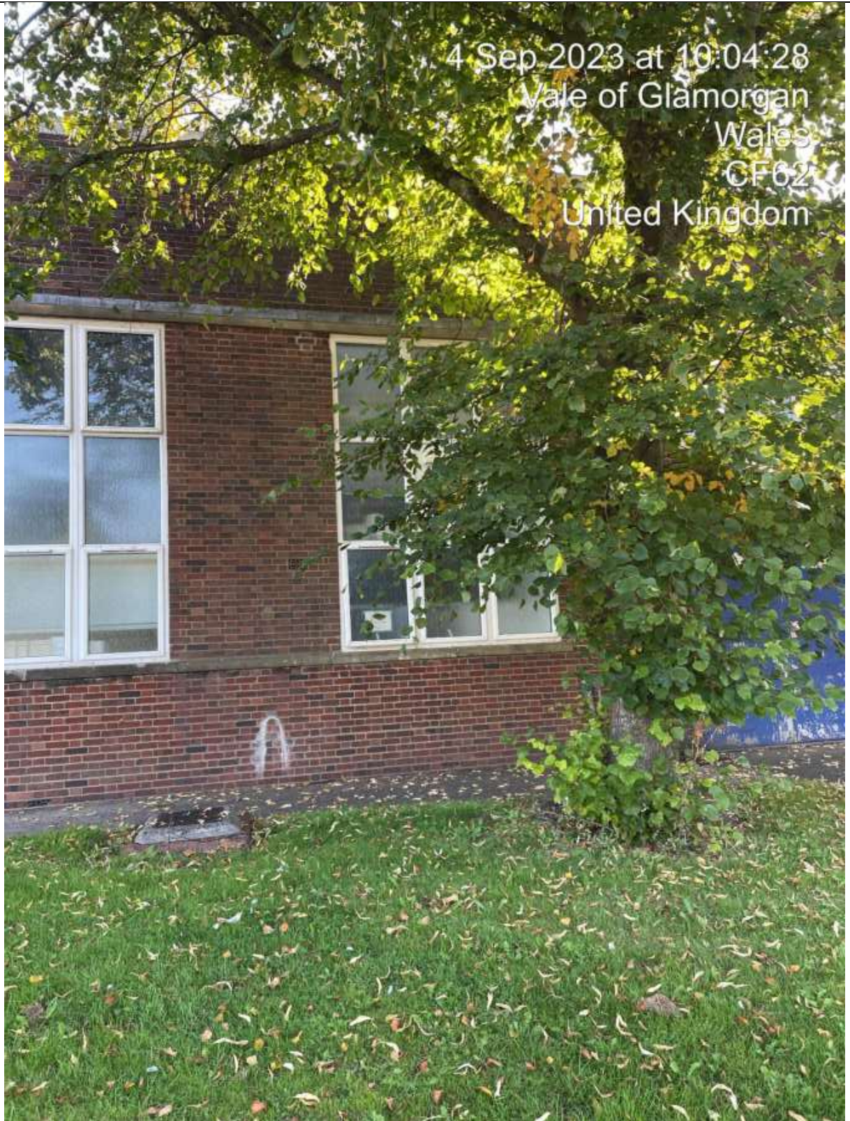
Western Elevation. Proximity of Trees to Building cause suspect of Damage to Foundations.
