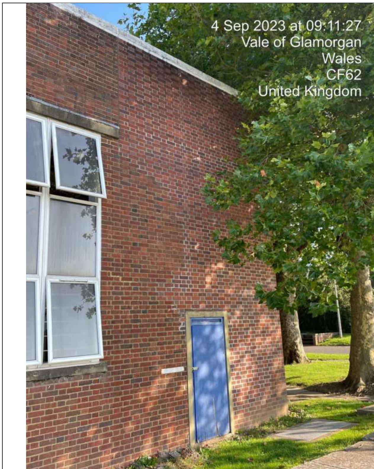
Southern Elevation. Note the Replacement Brickwork & Deterioration of Plant Room Door.
