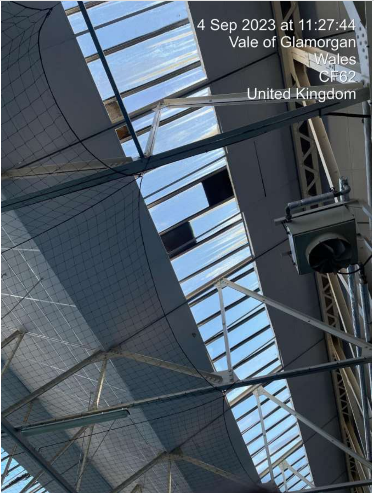
Damaged & Slipped Roof Lights.
