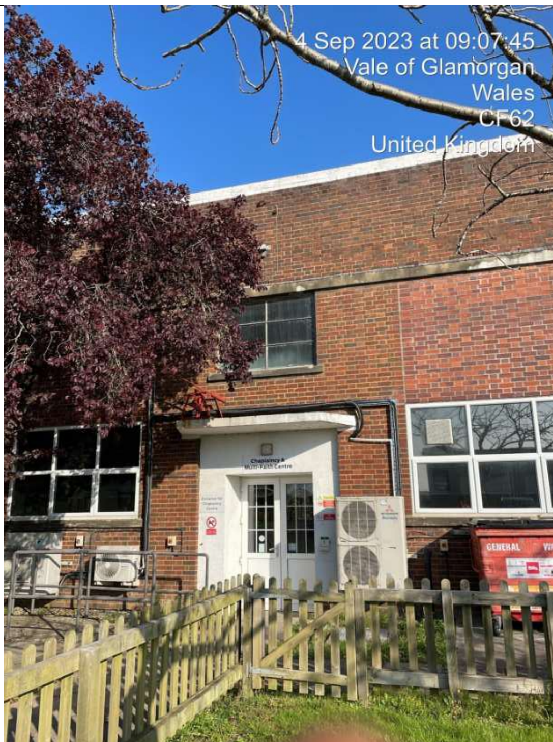
Southern Elevation. Note the Replacement Brickwork & Replacement Fenestration. Lack of Safety Covers Over Air Handling Units. Unprotected Switch Gear.
