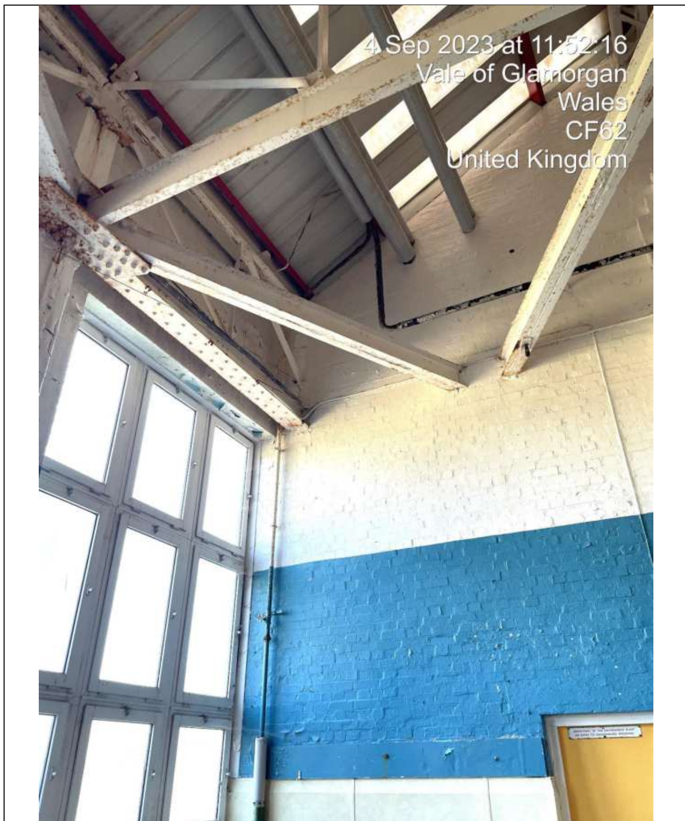
Corrosion to Steel Roof Frame. Penetrating Damp.
