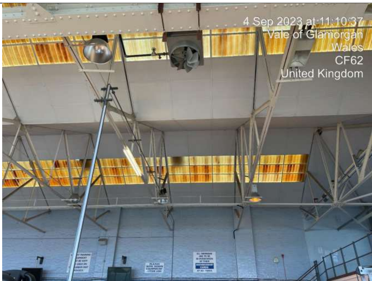
Discoloration to Roof Lights.
