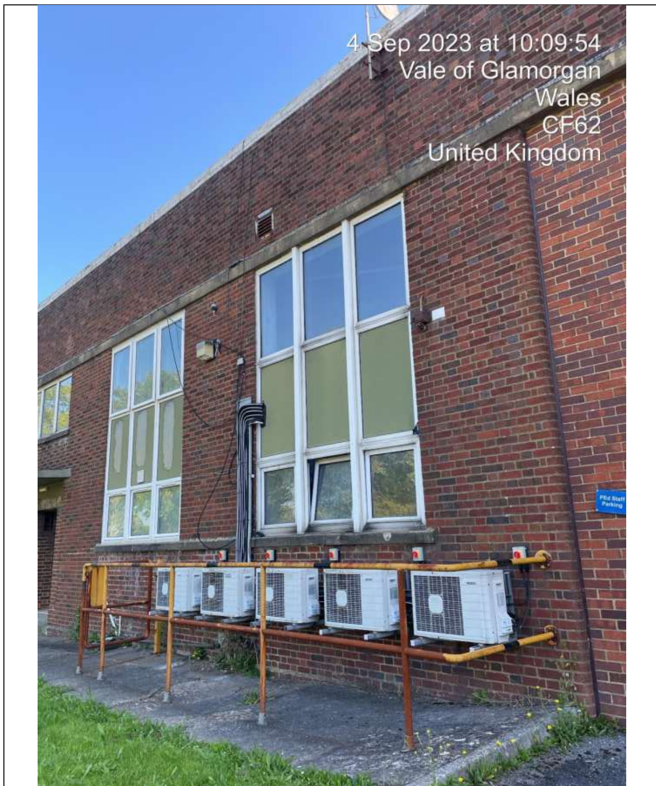
Western Elevation. Lack of Safety Covers Over Air Handling Units. Unprotected Switch Gear.
