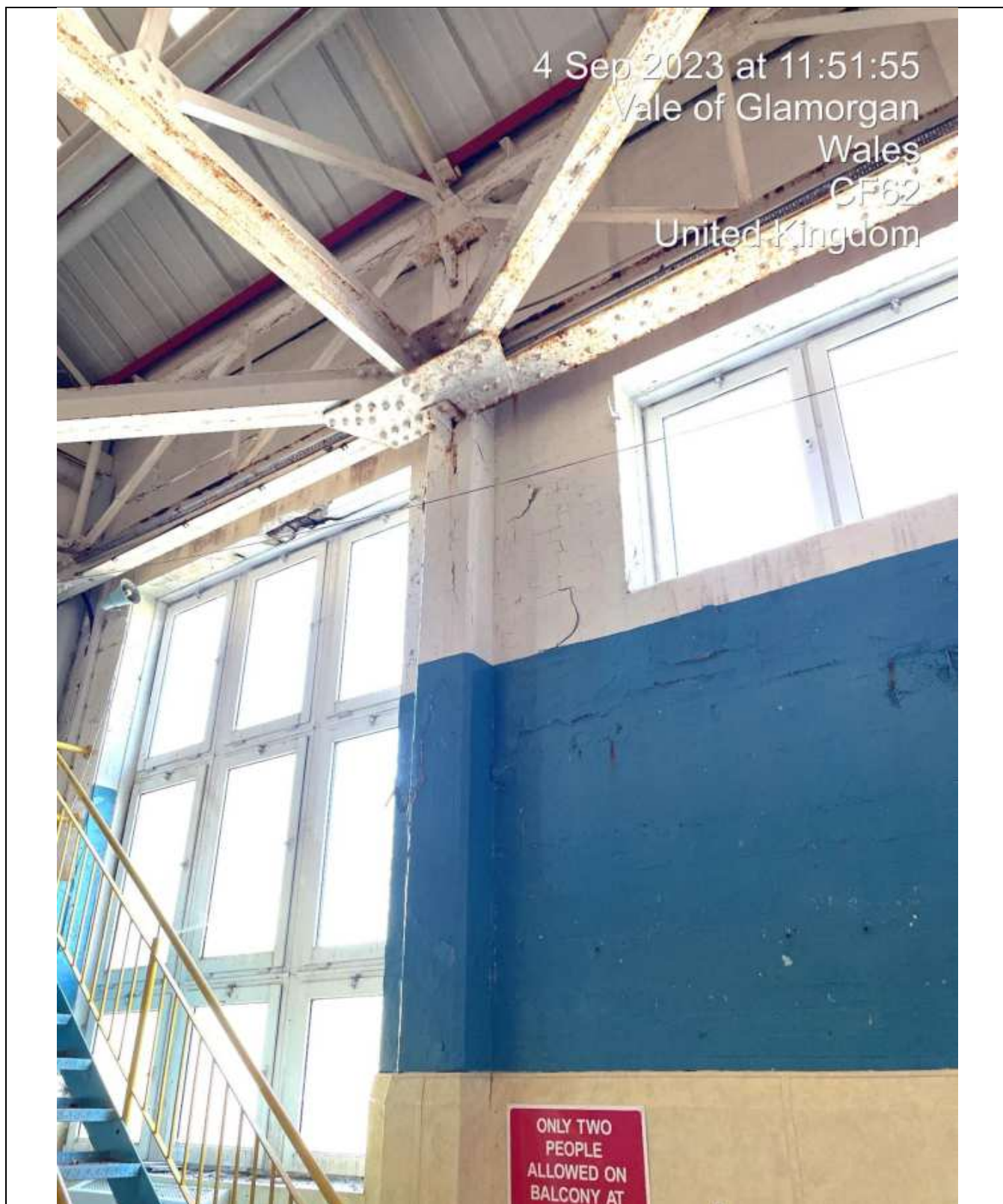
Corrosion to Steel Roof Frame. Penetrating Damp. Partial COLLAPSE of Lintel over Window.
