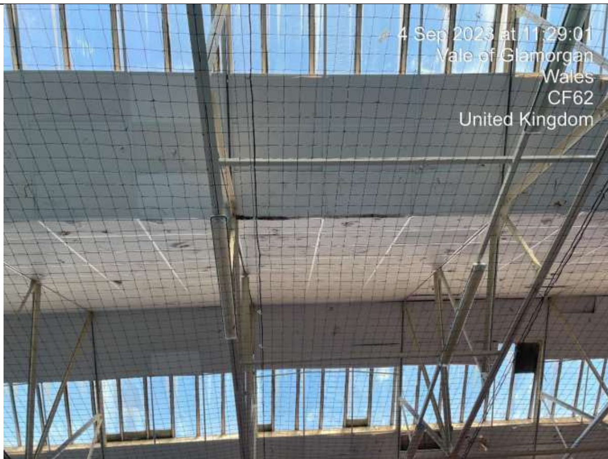
Deterioration to Suspended Ceiling Tiles.
