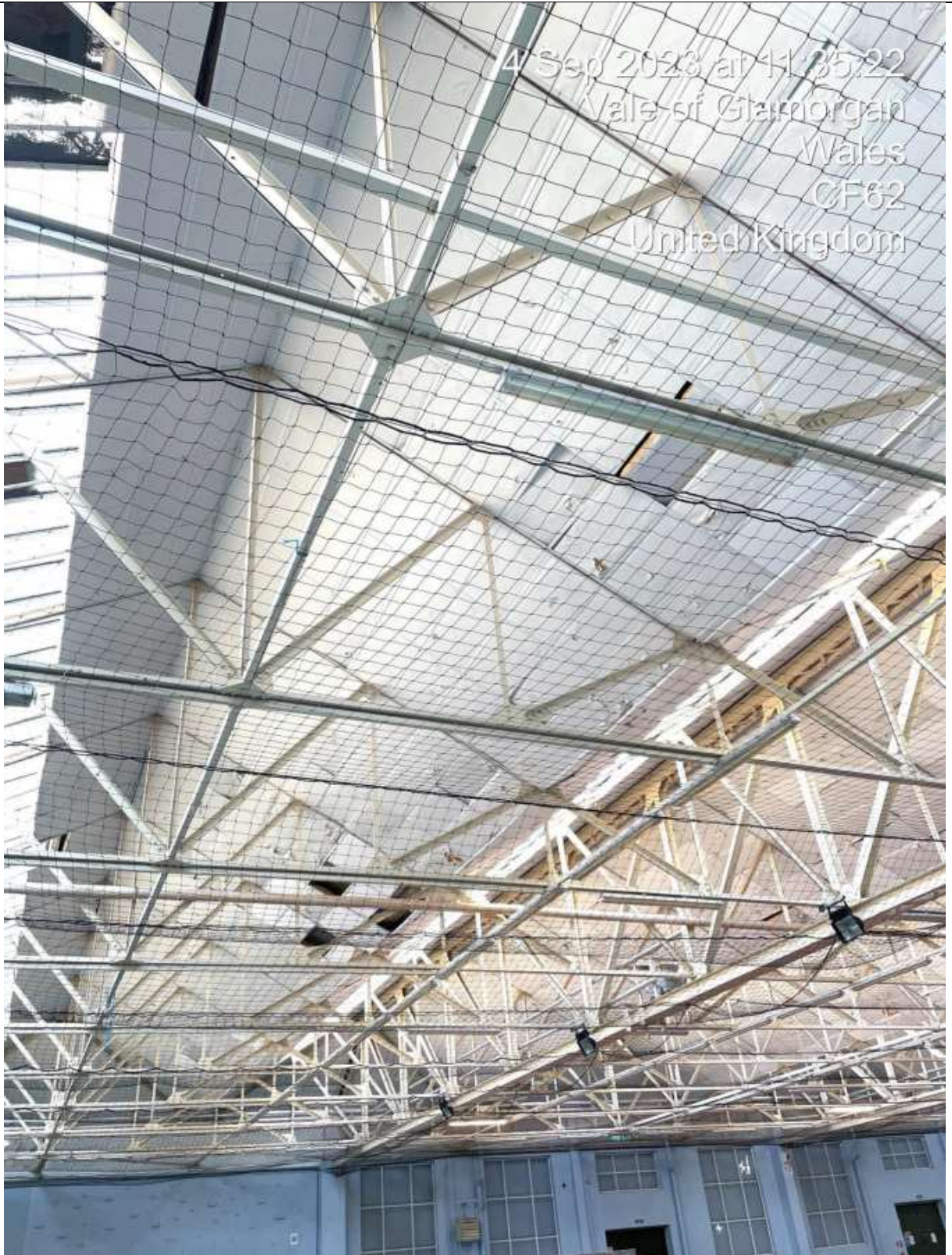
Deterioration & Missing Suspended Ceiling Tiles.
