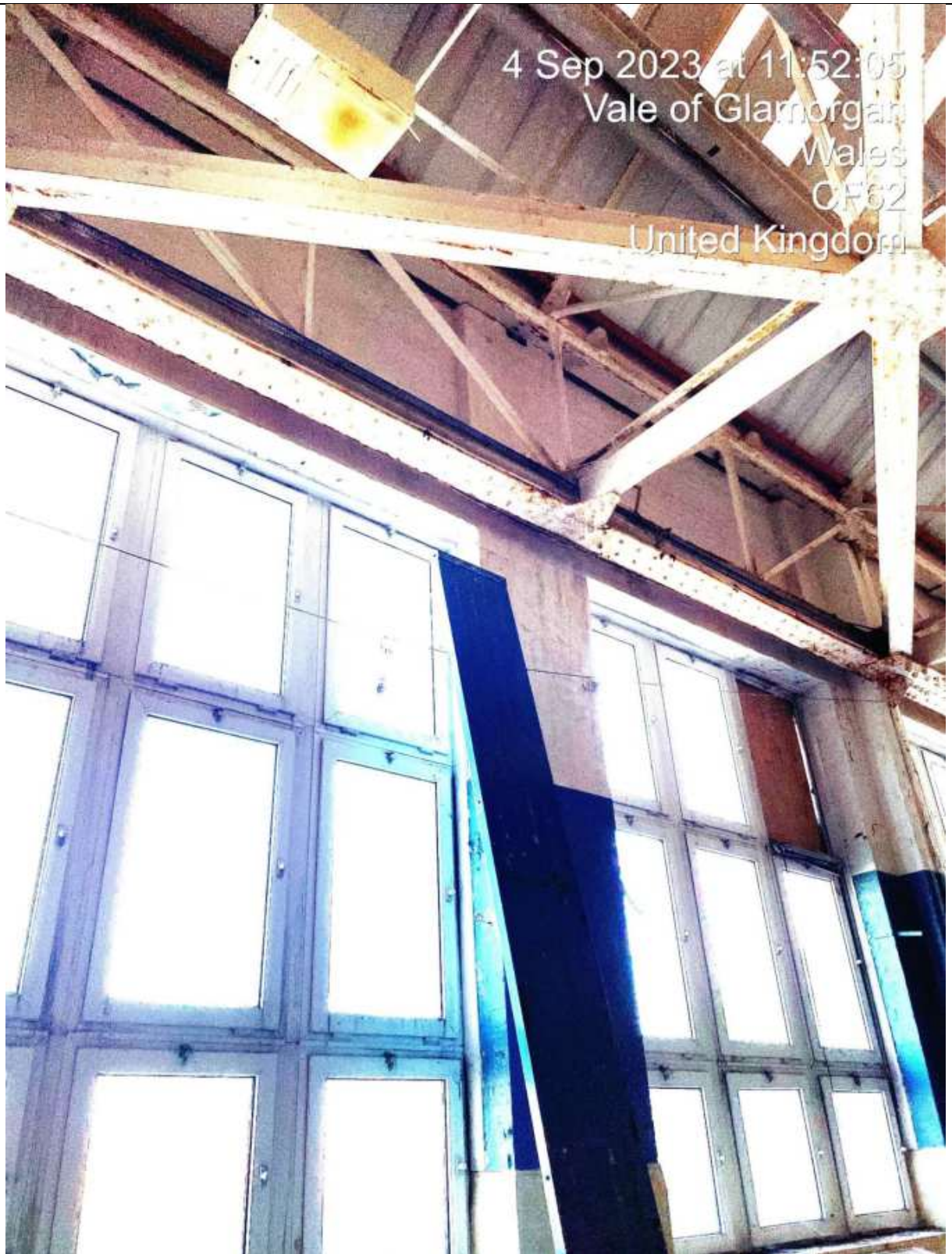
Corrosion to Steel Roof Frame & MISSING Glazing to Fenestration.
