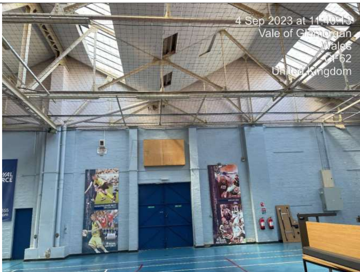
Deterioration & Missing Suspended Ceiling Tiles.
