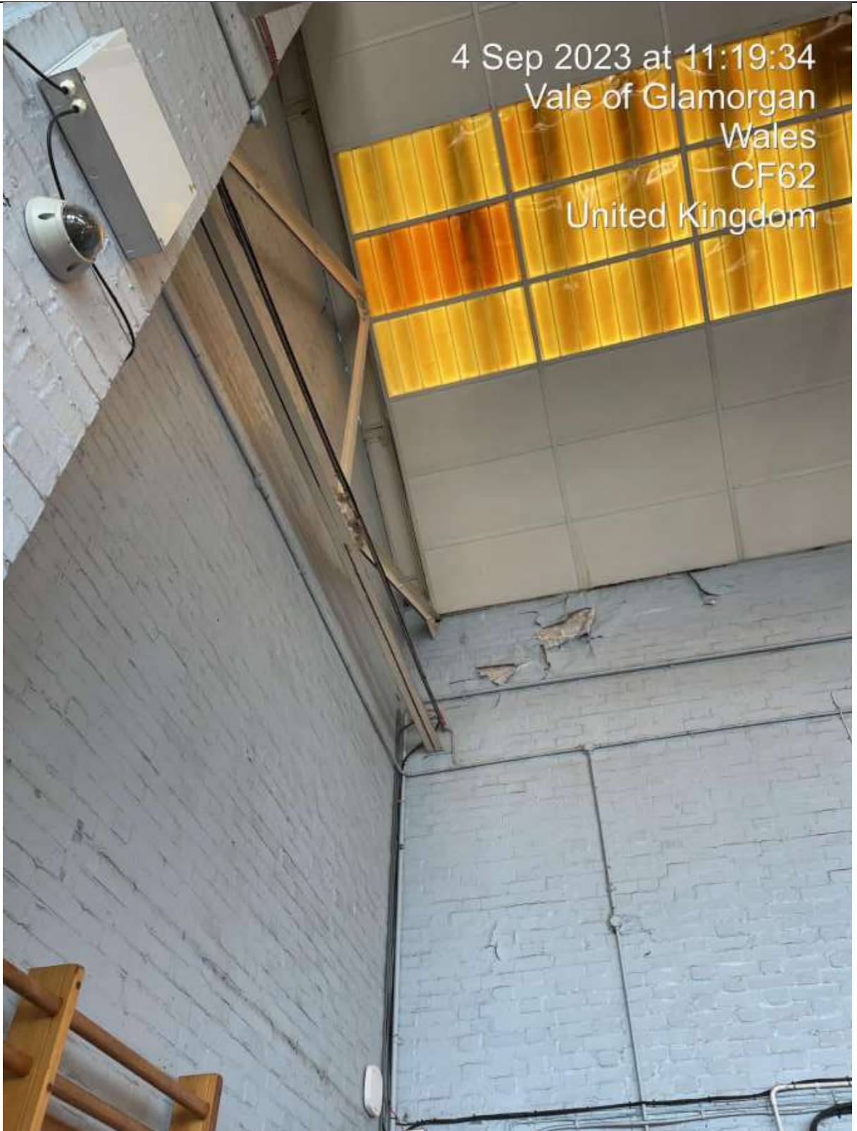
Penetrating Damp & Discoloration to Roof Lights.
