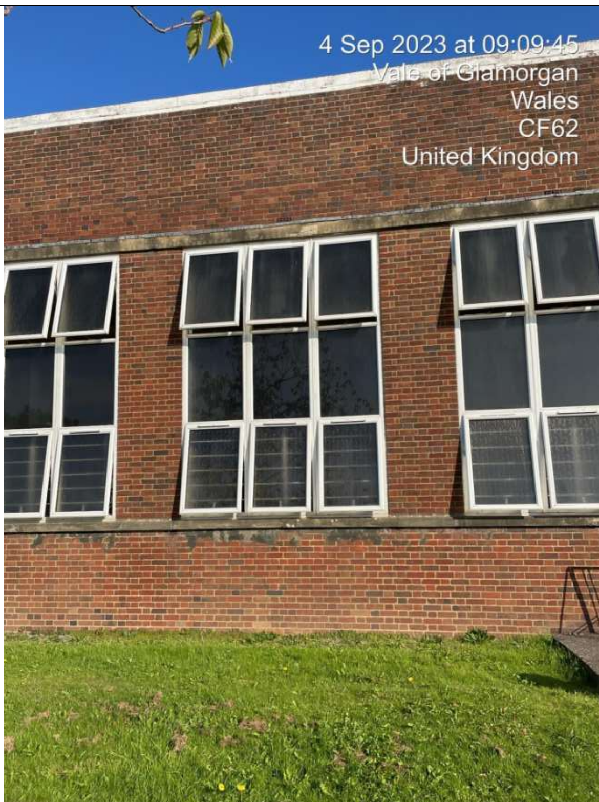
Southern Elevation. Replacement Fenestration.
