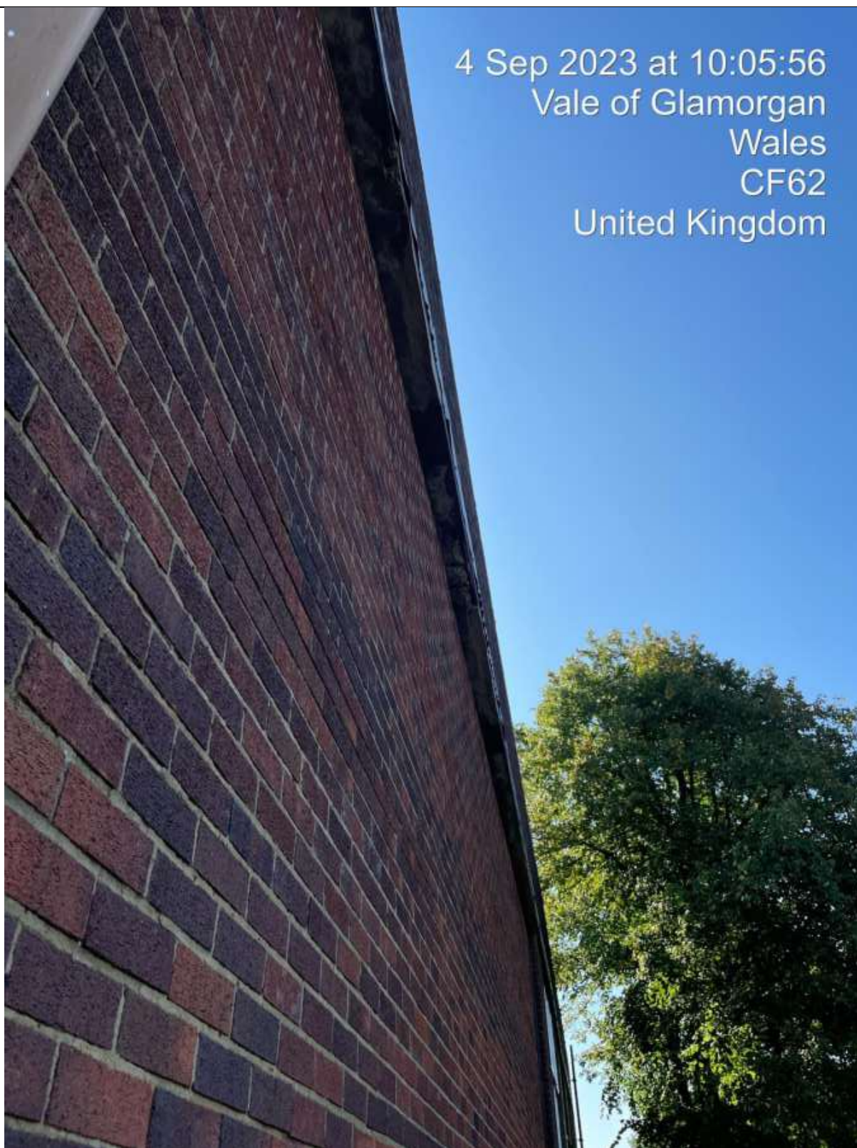
Western Elevation. Deterioration to Lintel.
