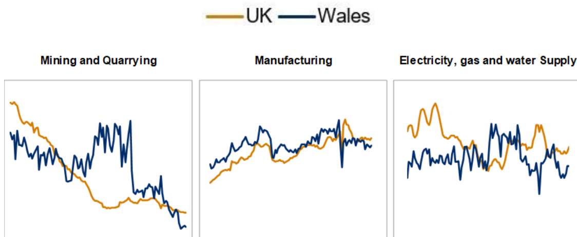
Figure 5.1: Production sub-indices – 1999 Q1 to 2025 Q1, (2022=100)
