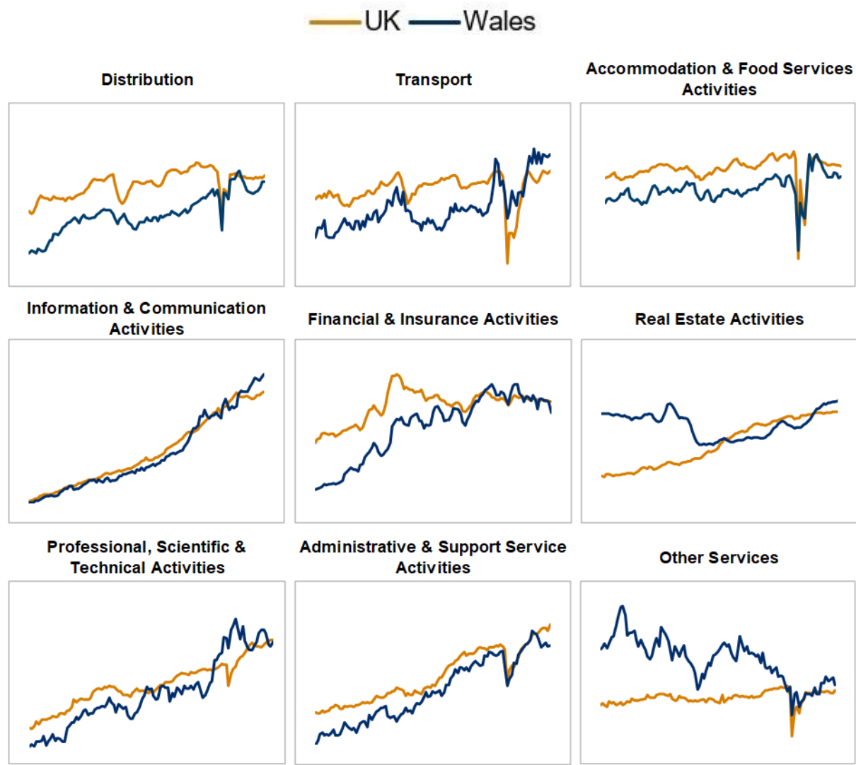
Figure 3.1: Market Services sub-indices – 1999 Q1 to 2025 Q1, (2022=100)
